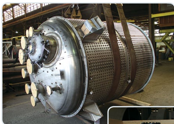
96' O.D x 144" OAH Jacketed process vessel
