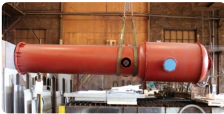
Amonia separator
